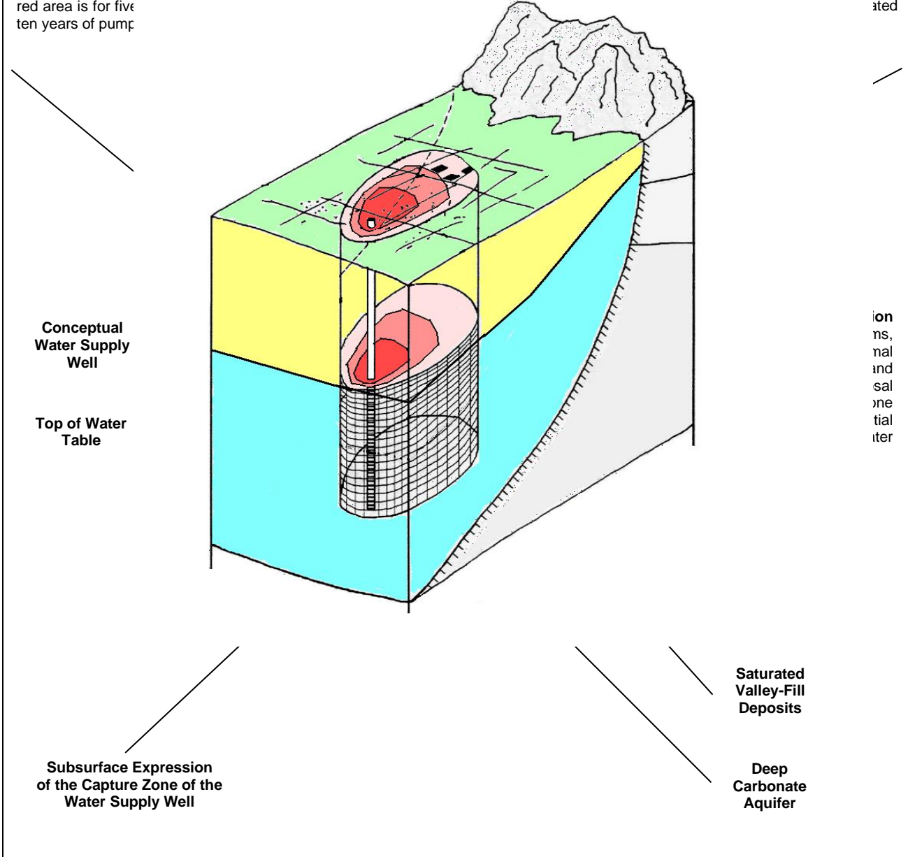
Figure 9. Conceptual Drawing of the Wellhead Protection Areas for District Water Supply Wells and Springs. Modified from Bureau of Water Quality Planning Guidance Document.
